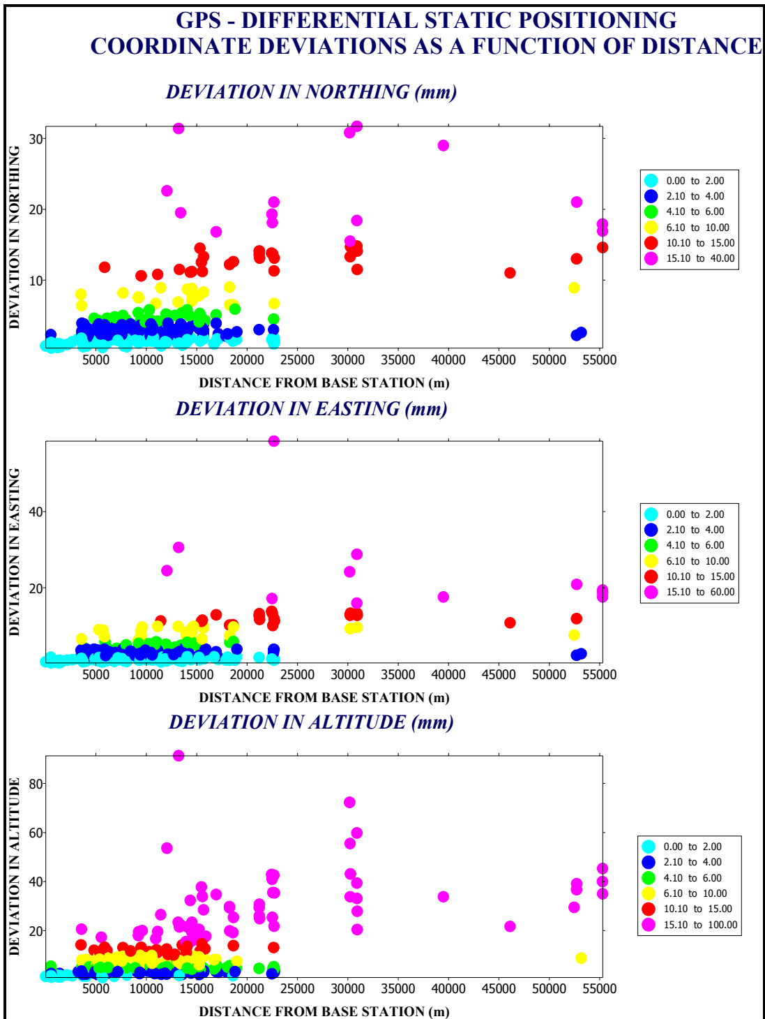
Figure 10 : Representation of the deviations in the three dimensions as a function of distance
