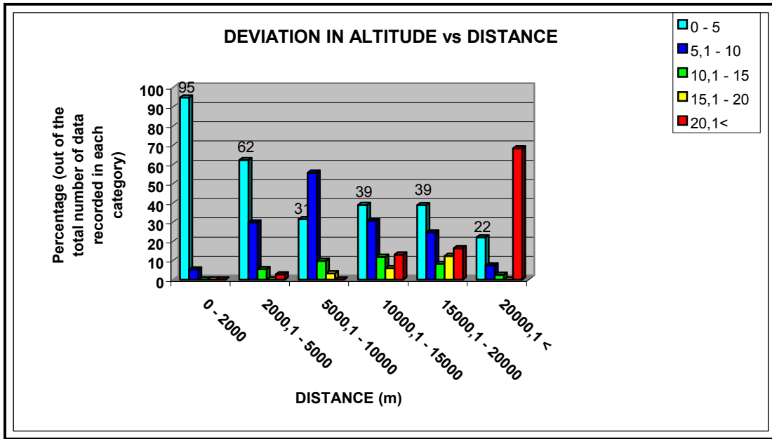
Figure 7 : Deviation in Altitude (z) vs Distance
