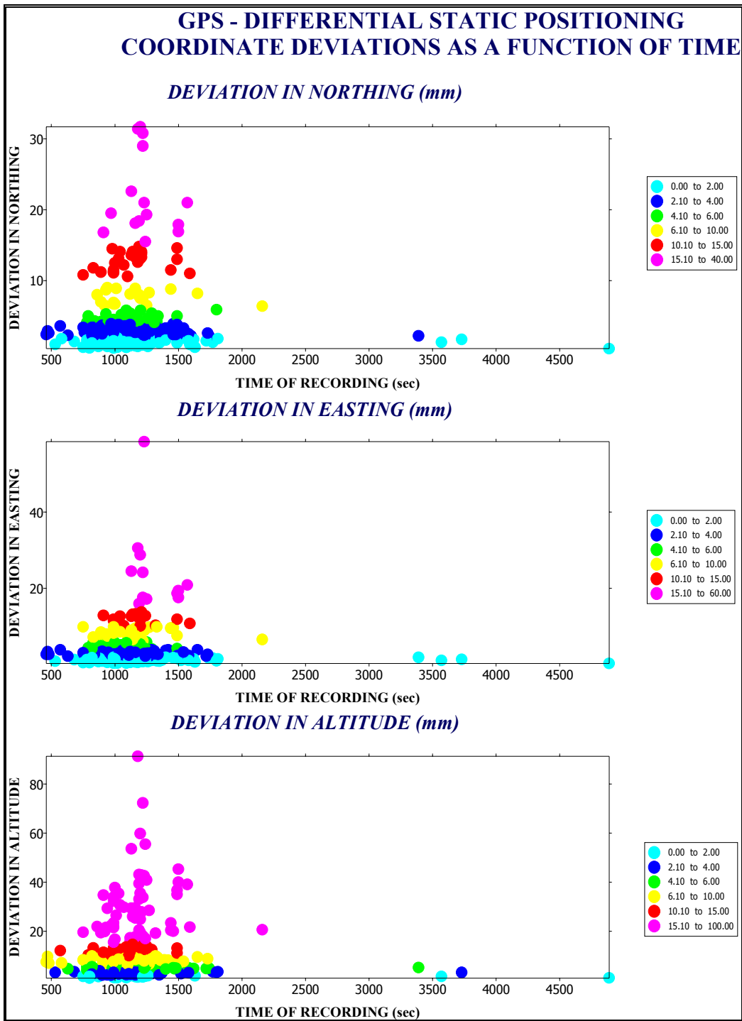
Figure 9 : Representation of the deviations in the three dimensions as a function of time
