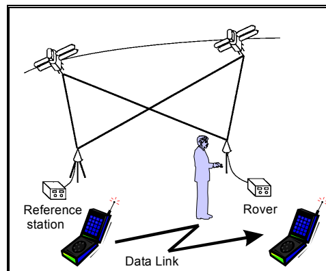
Figure 3 Real Time Kinematic GPS
