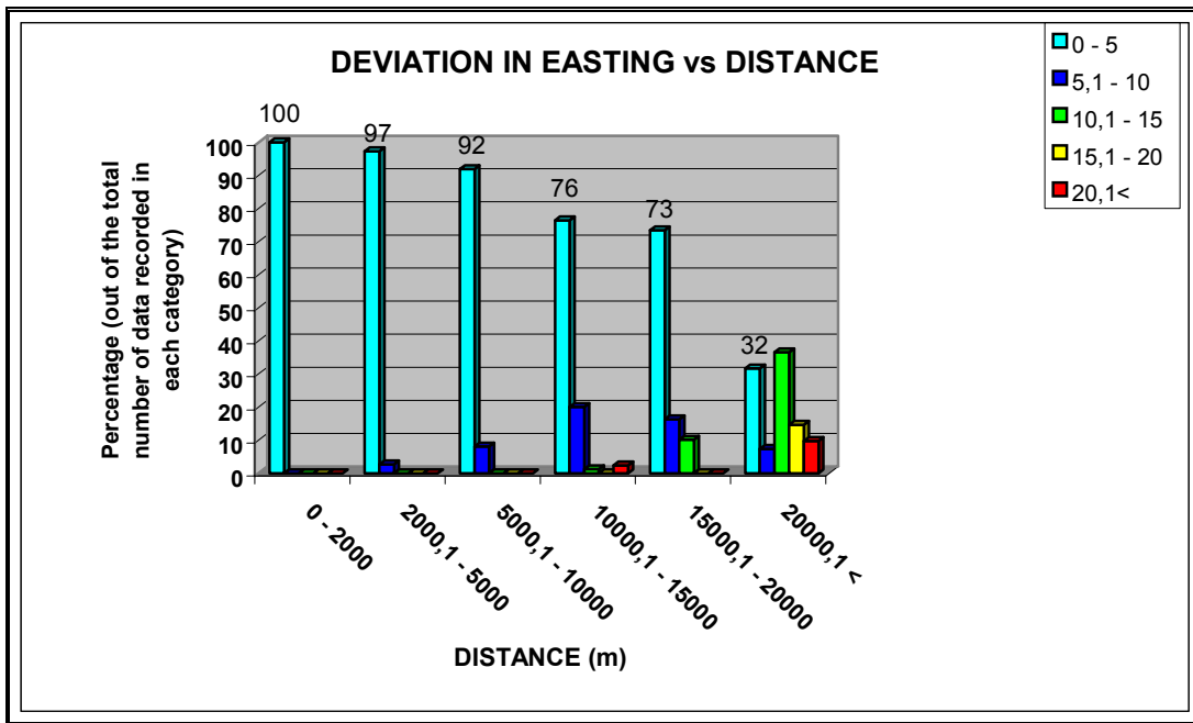
Figure 5 : Deviation in Easting (x) vs Distance
