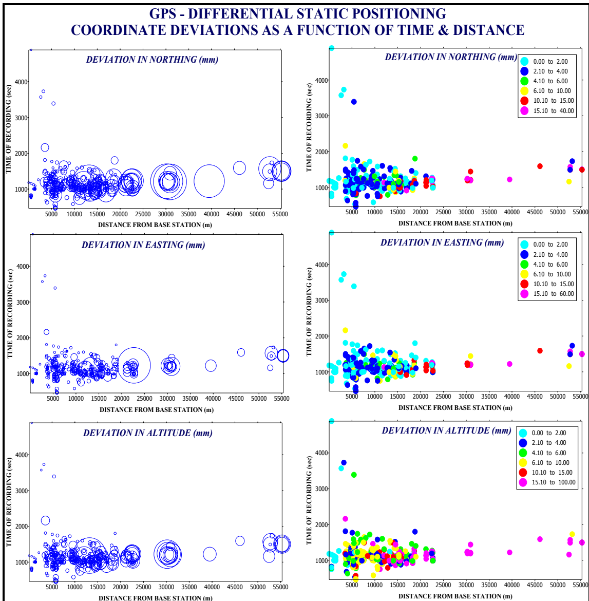
Figure 8 : Correlation of observation time, distance and deviation in the three dimensions. Representation of error in graduation of shape size (left) and color (right).
