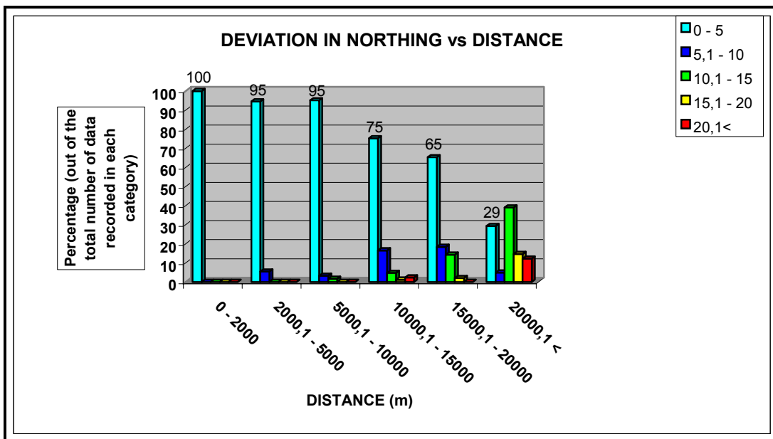
Figure 6 : Deviation in Northing (y) vs Distance
