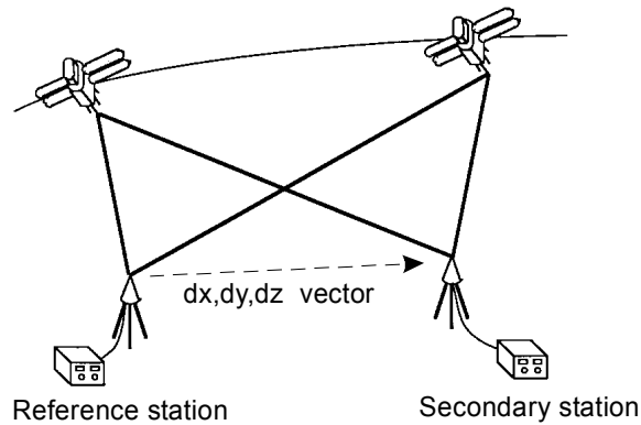
Figure 2: Relative static positioning
